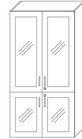
MATERIALSKÅP MS4G 4ST GLASADE LUCKOR L800, 1000 H1950 D450
